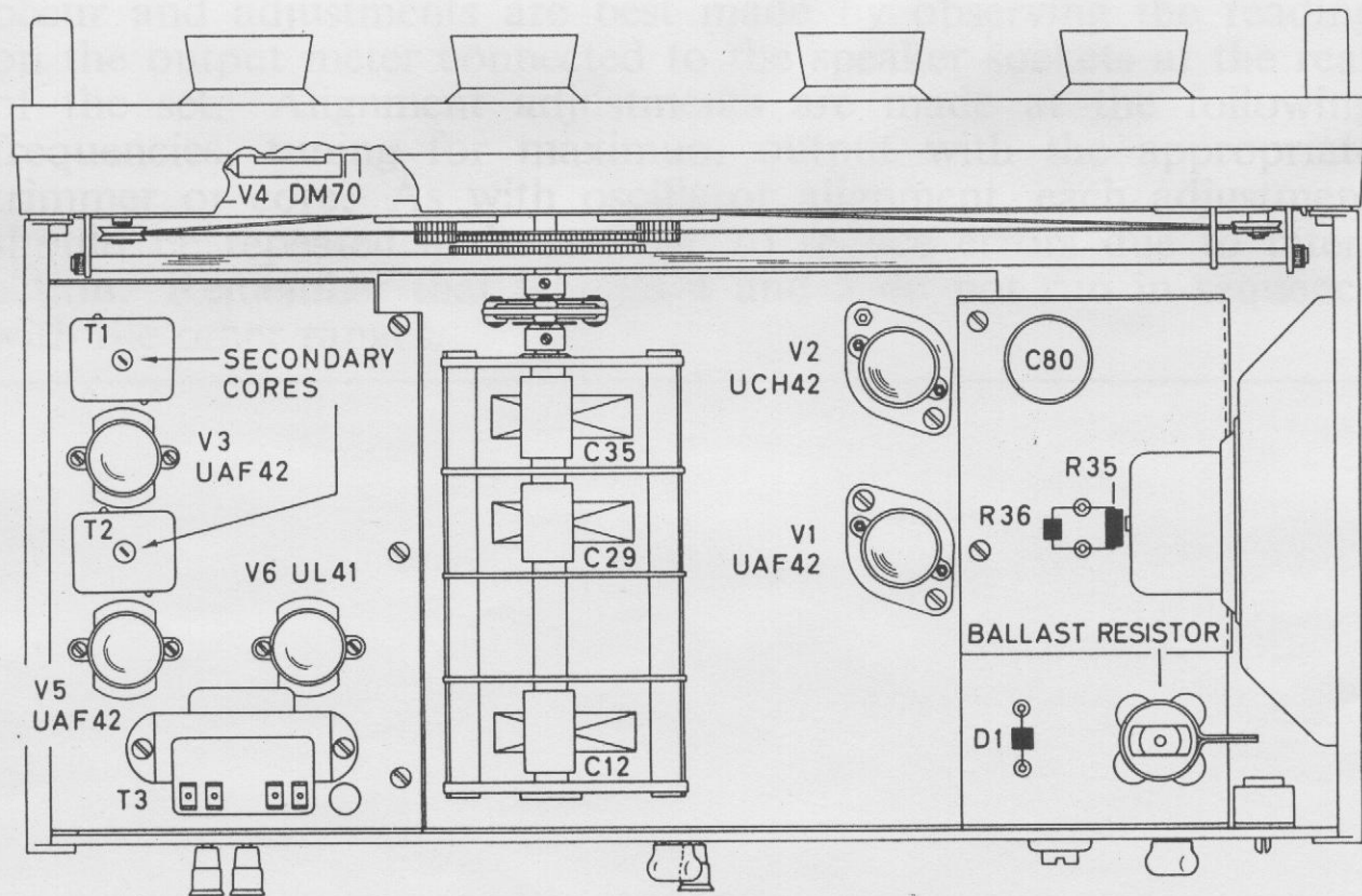
Plan view of receiver
